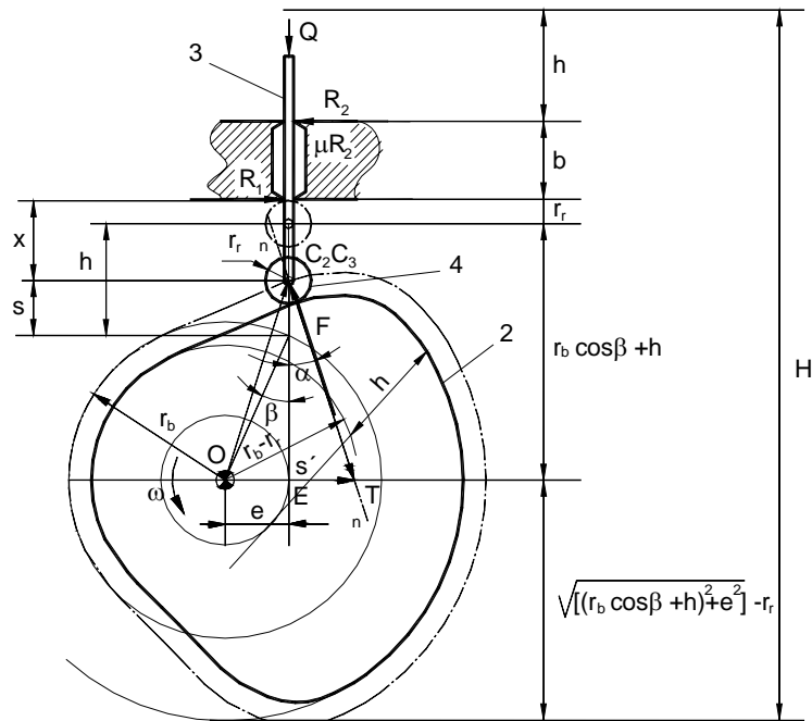
Fig. 1. The geometry, kinematics and forces equilibrium on a current position of a cam mechanism with roll translating follower
